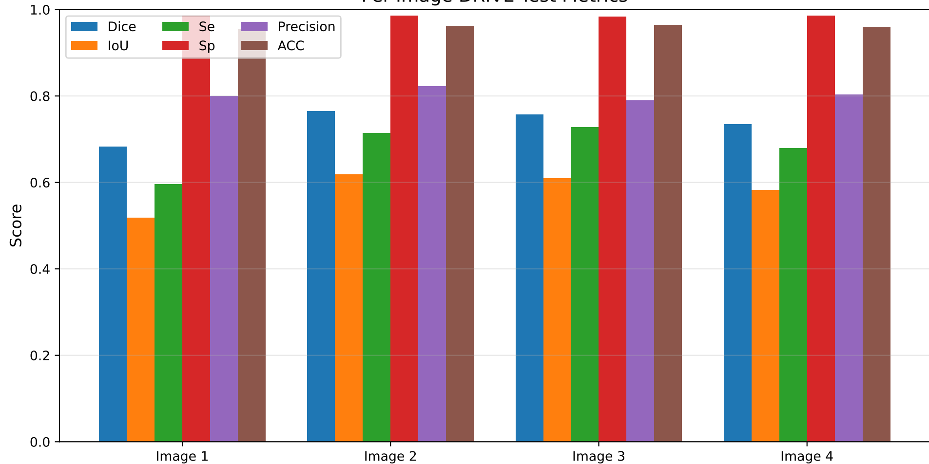
Per-Image DRIVE Test Metrics
