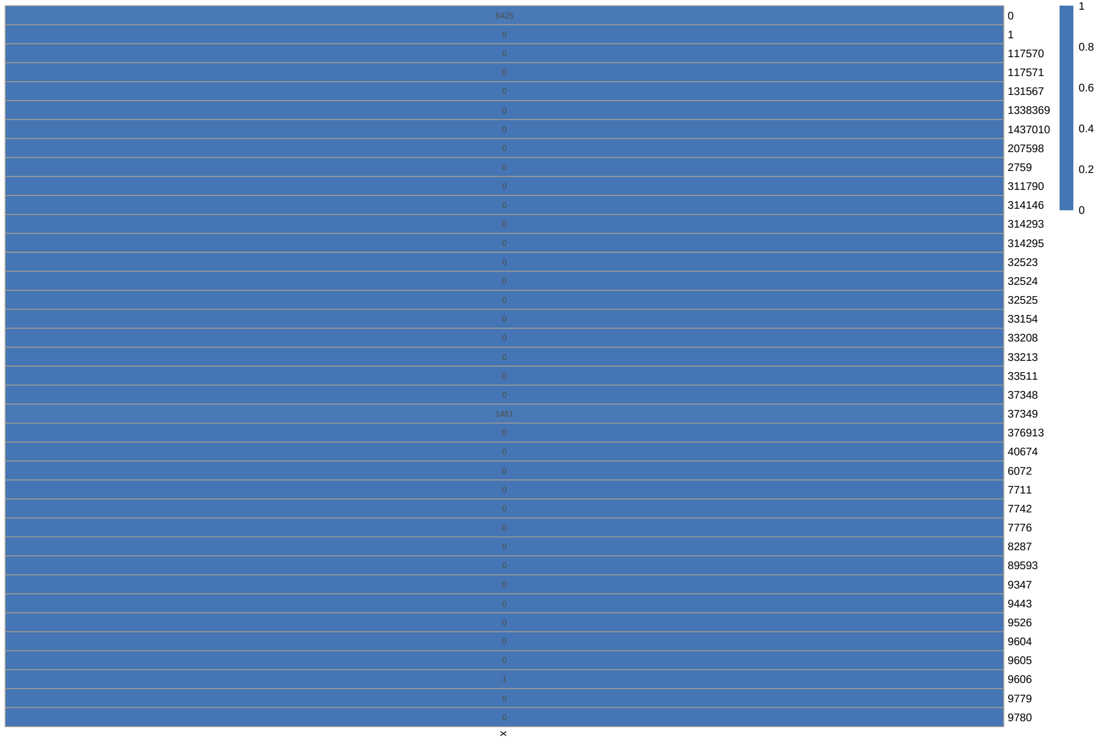
KrakenUniq Absolute Abundance
