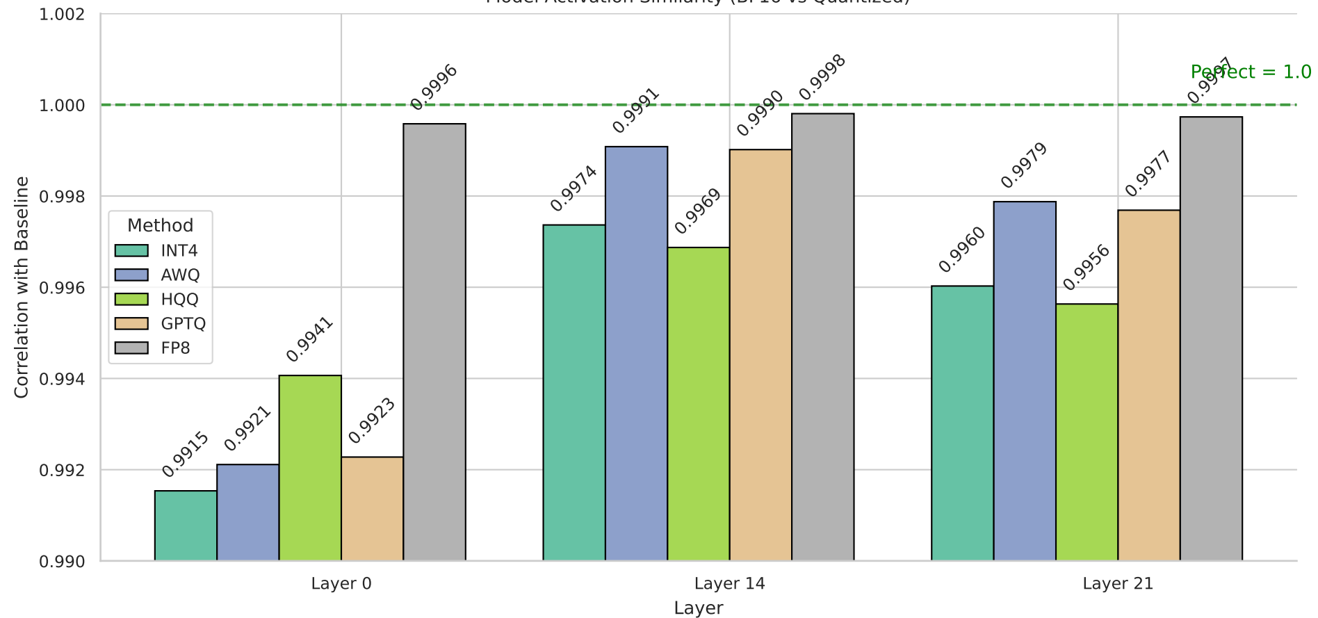
Model Activation Similarity (BF16 vs Quantized)
