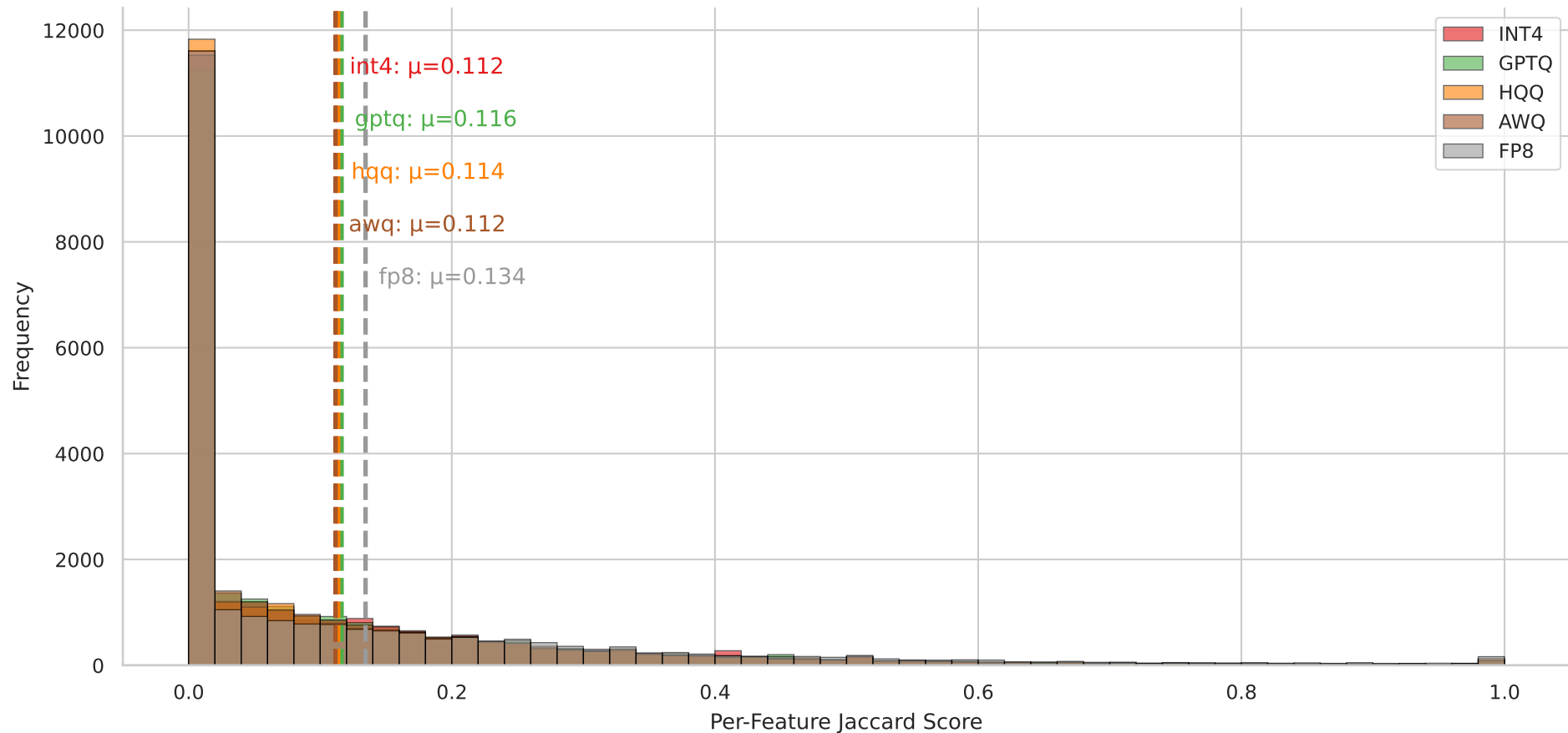
Distribution of Functional Jaccard Scores
