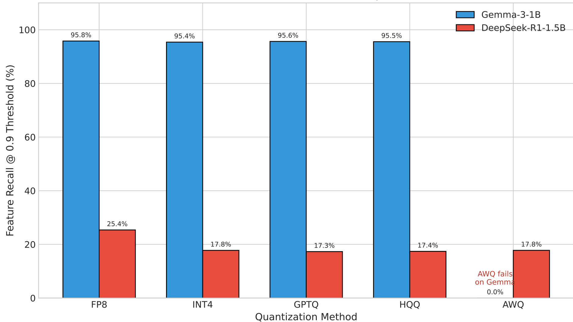
SAE Feature Preservation: Architecture-Dependent Results
