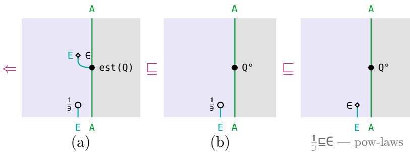
(a) \triangleq \text{thin}, \in \setminus (Q^\circ \in) half
