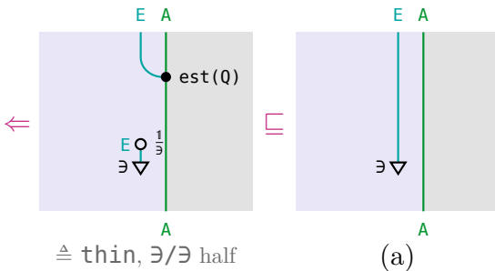
(a) \frac{1}{\exists} \sqsubseteq 1 — \text{pow-laws} ; \text{est}(Q) \sqsubseteq \exists — \text{est-laws}
