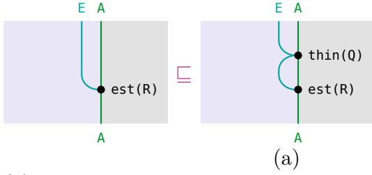
(a) 1 \sqsubseteq \text{thin}(Q) — (14.1b)
