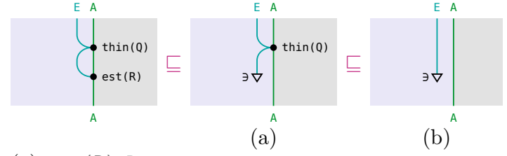
(a) \text{est}(R) \sqsubseteq \exists — \text{est-laws}
