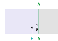
the A \times - summand: \exists picks one path, 1\% \exists collects the results
