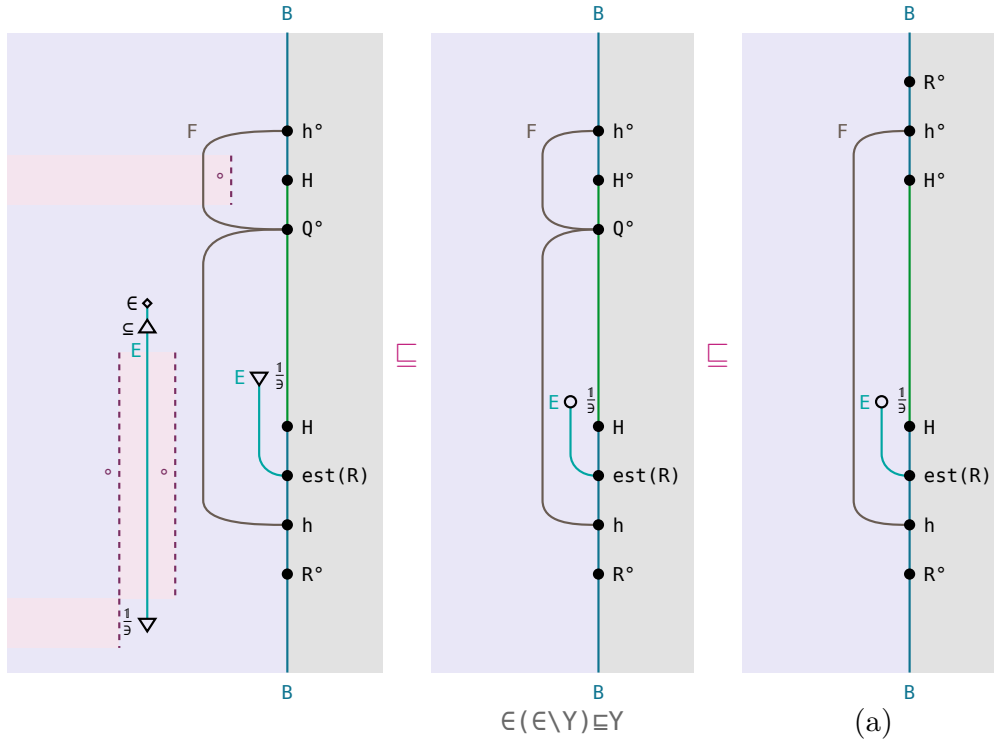
(a) QF(H)h \sqsubseteq F(H)hR conversed
