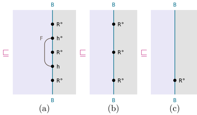
(a) H^\circ M \sqsubseteq R^\circ under F — est-up
