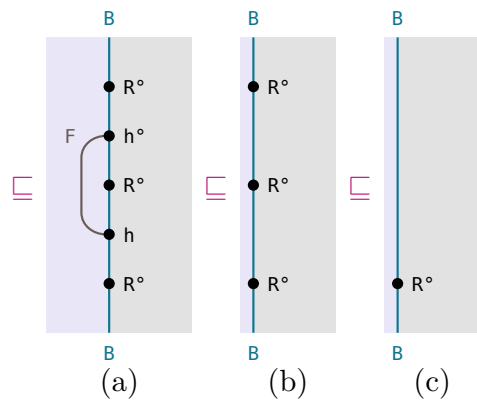
(a) H^\circ M \sqsubseteq R^\circ under F — (7.1.1a)
