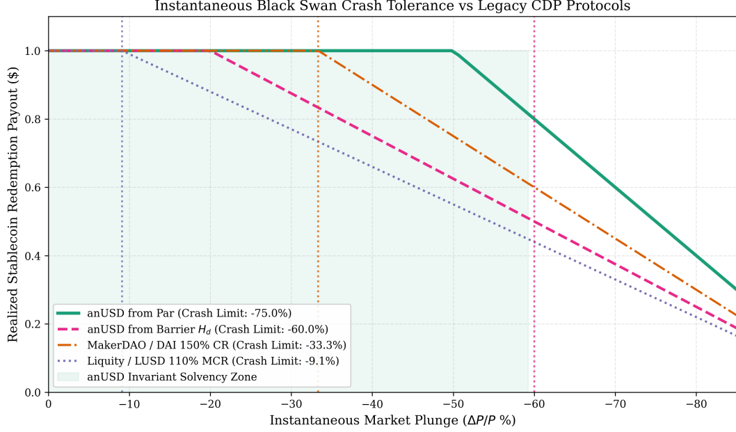
Figure 3: Instantaneous Black Swan flash-crash stress test comparing realized redemption payouts across stablecoin protocols. anUSD maintains 100% par redemption for instantaneous market drops up to -60.0\% from the lower barrier H_d (and -75.0\% from par), substantially outperforming MakerDAO DAI ( -33.3\% ) and Liquity LUSD ( -9.1\% ).
