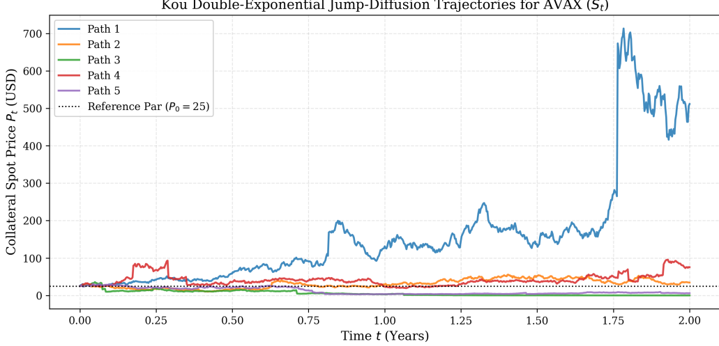
Figure 4: Monte Carlo simulated trajectories of AVAX collateral spot price ( S_t ) under Kou's double-exponential jump-diffusion process ( \sigma = 75\% , \lambda = 3.5 , p = 0.40 , \eta_1 = 3.5 , \eta_2 = 2.0 ) over a 2-year simulation horizon.
