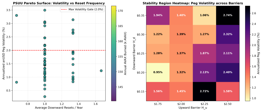
Figure 8: Multi-Objective PSUU Pareto Frontier mapping trade-offs between Annual Peg Volatility ( \leq 2.00\% ), Reset Friction Frequency ( < 3.0/\text{year} ), and Protocol Capital Efficiency. The optimal design corridor \theta^* = (R = 7.30\%, H_u = \$2.00, H_d = \$0.25) achieves the Pareto-optimal balance.
