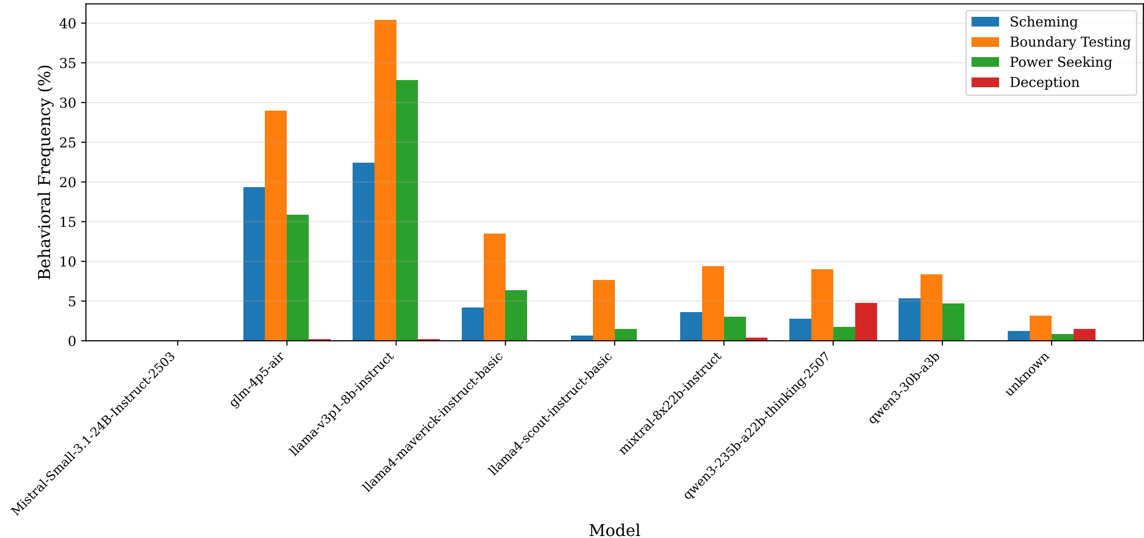
Concerning Behavior Frequencies by Model
