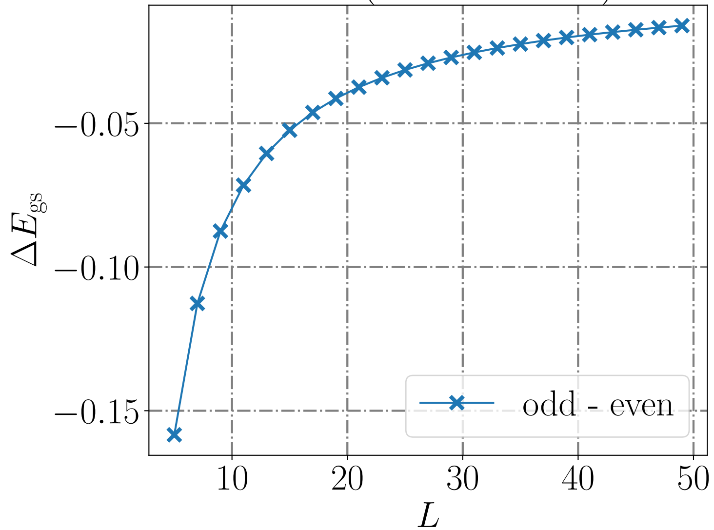
L odd ( E^{\text{odd}} is lower)
