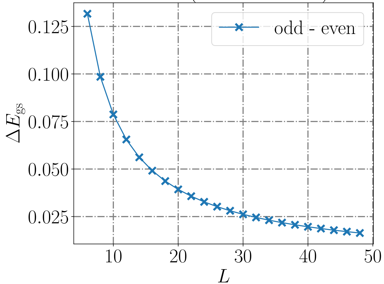
L even ( E^{\text{even}} is lower)
