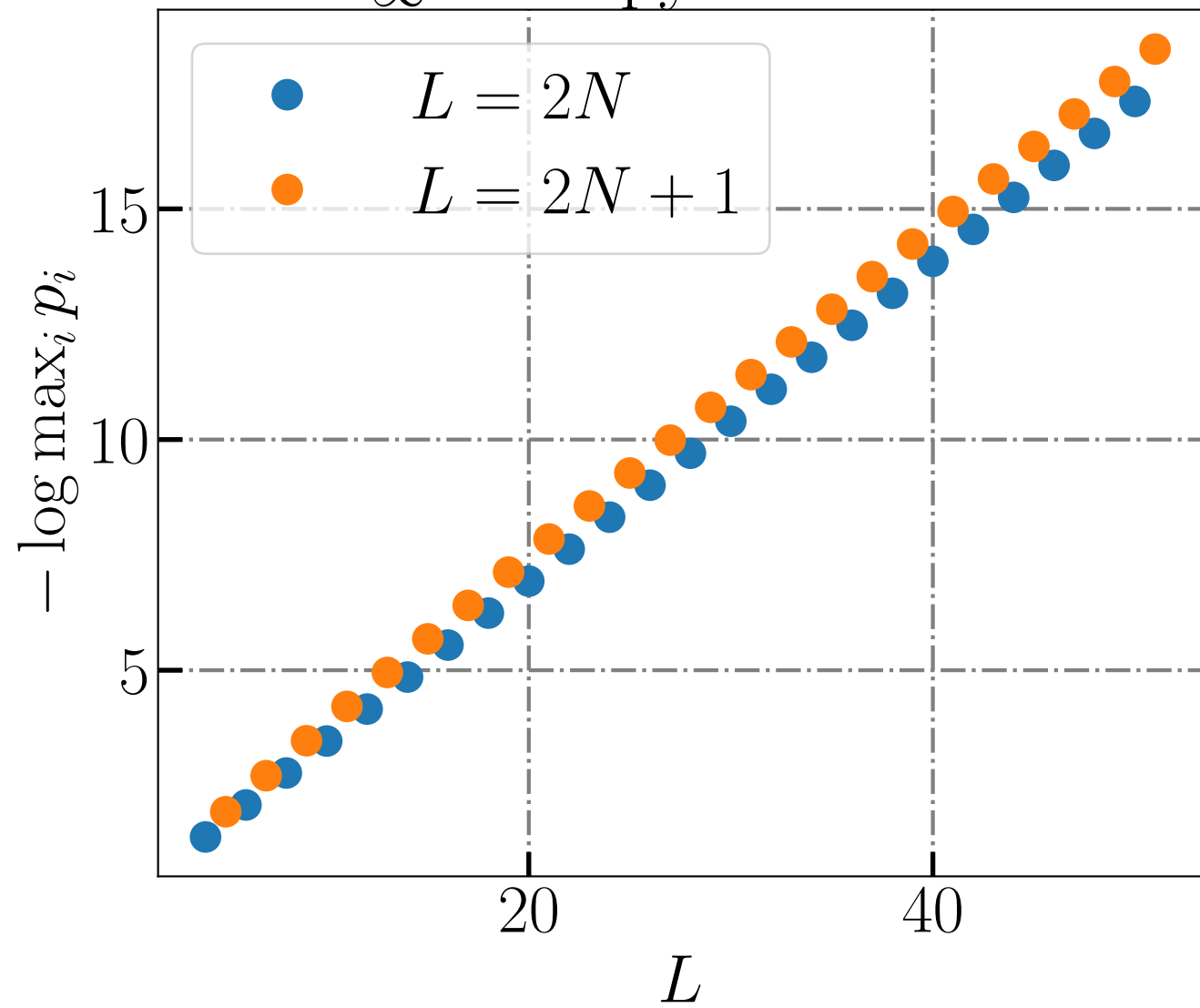
S_\infty entropy for \Delta = 0
