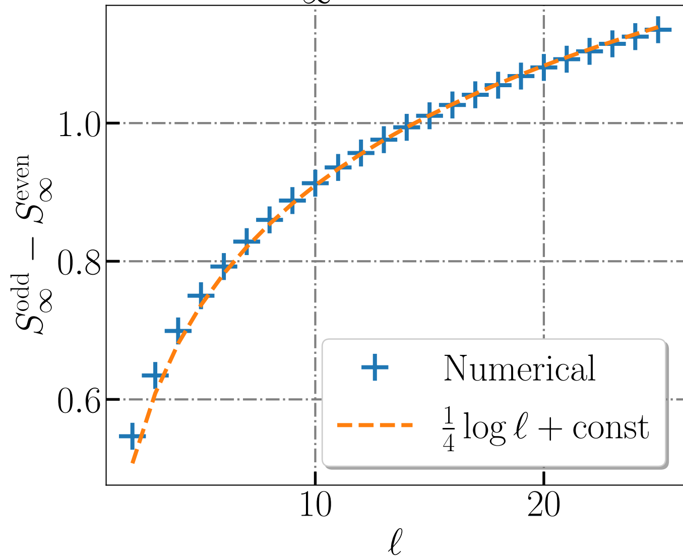
S_\infty difference
