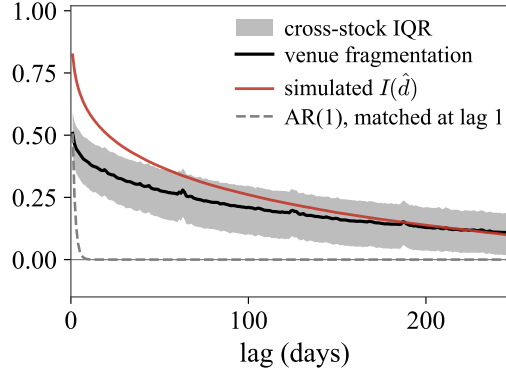
(E) Cross-sectional ACF of Daily Fragmentation
