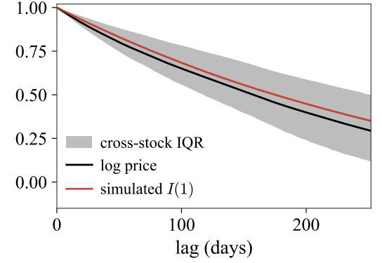
(F) Cross-sectional ACF of Daily Log Price
