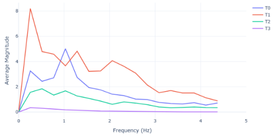
FFT Bin Averaged Plot - 35% Duty Cycle, No Net
