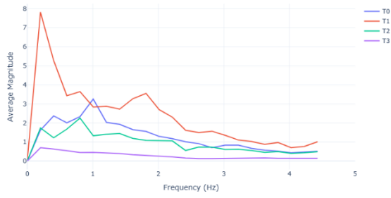
FFT Bin Averaged Plot - 25% Duty Cycle, No Net
