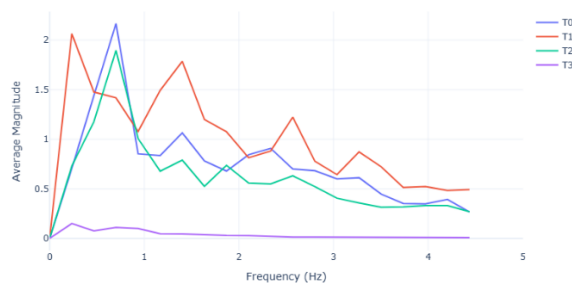
FFT Bin Averaged Plot - 10% Duty Cycle, With Net
