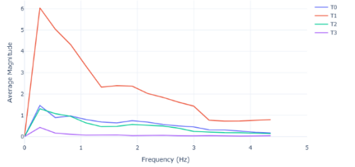
FFT Bin Averaged Plot - 40% Duty Cycle, With Net
