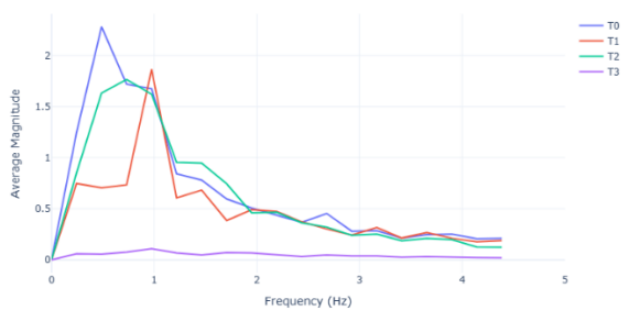
FFT Bin Averaged Plot - 5% Duty Cycle, No Net
