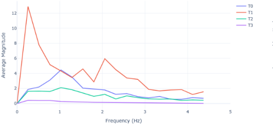
FFT Bin Averaged Plot - 40% Duty Cycle, No Net
