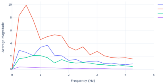
FFT Bin Averaged Plot - 35% Duty Cycle, No Net
