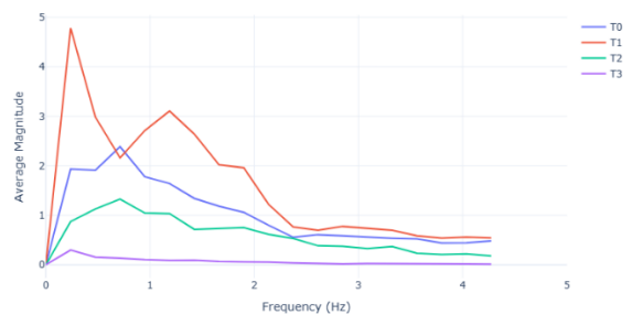
FFT Bin Averaged Plot - 20% Duty Cycle, With Net
