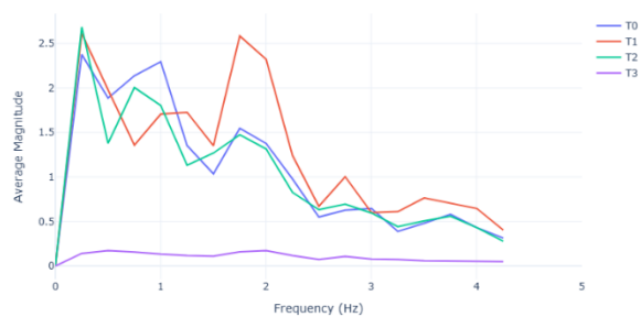
FFT Bin Averaged Plot - 15% Duty Cycle, No Net
