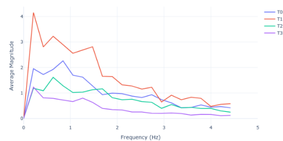
FFT Bin Averaged Plot - 20% Duty Cycle, No Net
