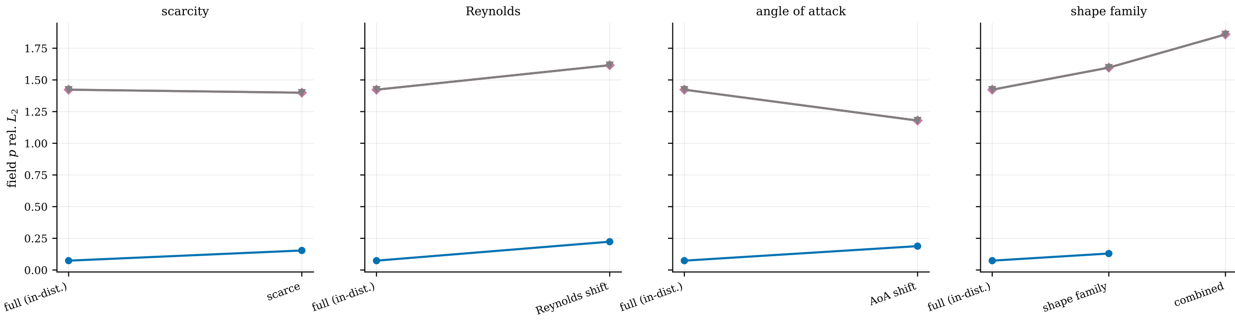
—●— M1 GNN —◆— Ridge —★— Constant Error vs distribution shift
