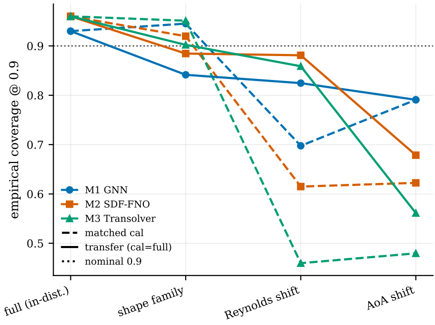
Coverage vs shift ( C_D^{\text{int}} )
