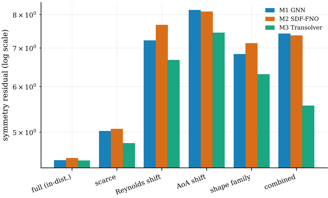
Symmetry (mirror-equivariance) violation, no augmentation
