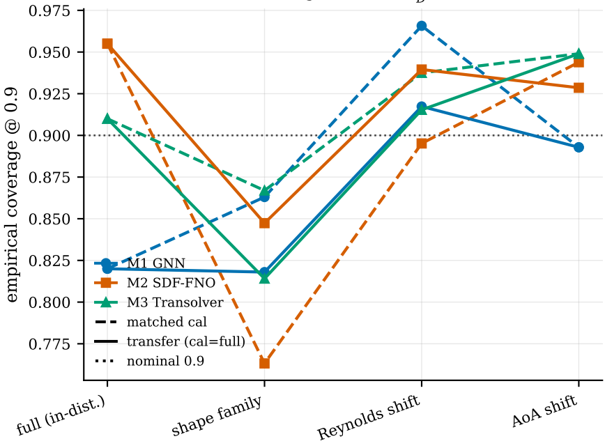
Coverage vs shift ( C_D^{\text{int}} )
