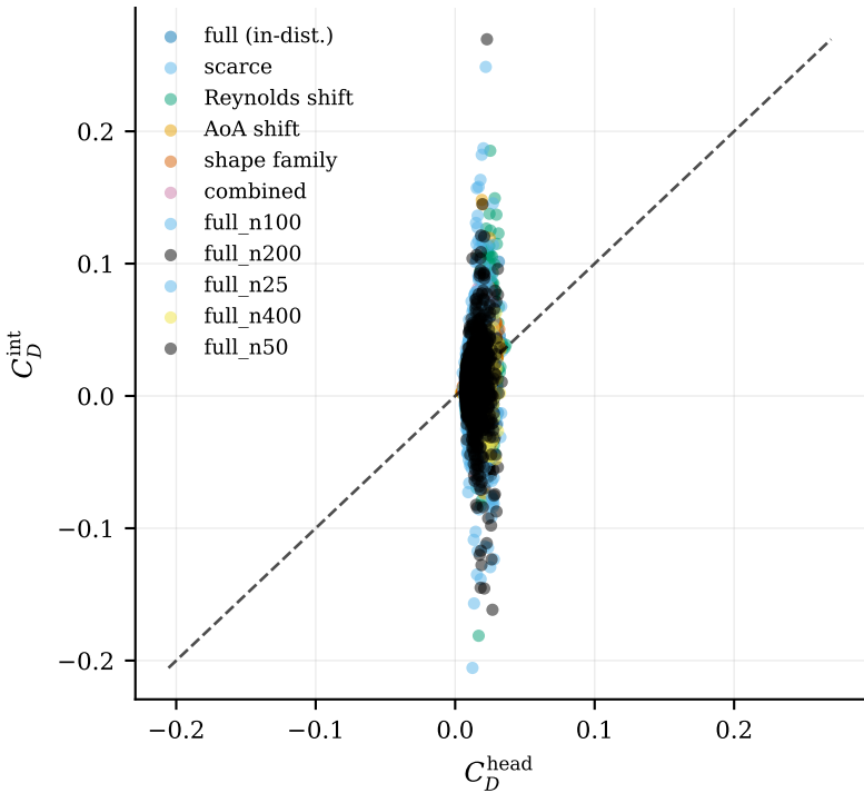
Force self-consistency
