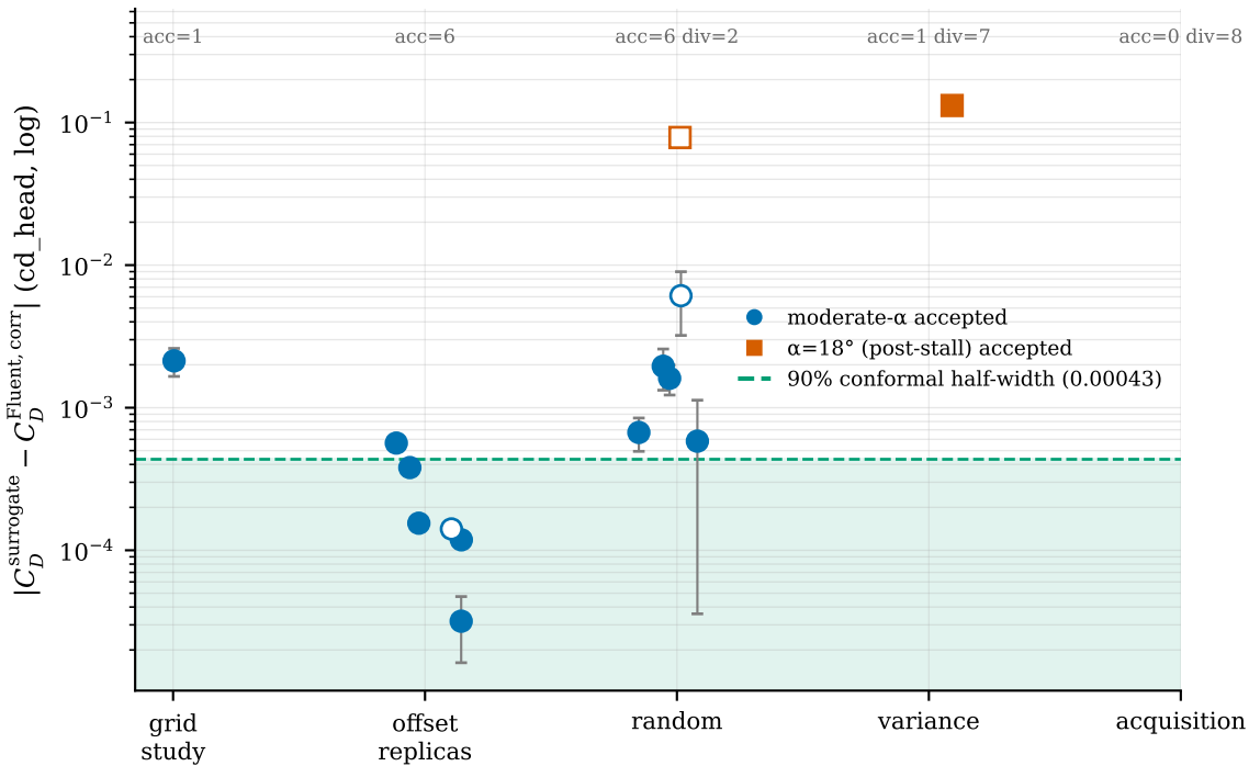
Surrogate vs Fluent by arm (accepted set); markers = post-stall regime
