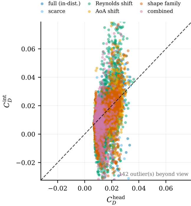
FIG. 5. Force self-consistency: C_D^{\text{int}} against C_D^{\text{head}} , one point per test simulation pooled over all three models, coloured by split, against the identity line (axes zoomed to the central 99% of the data). Distance from the identity line is FSC; the vertical spread at fixed C_D^{\text{head}} is the integrated route disagreeing with the head it shares a backbone with.
