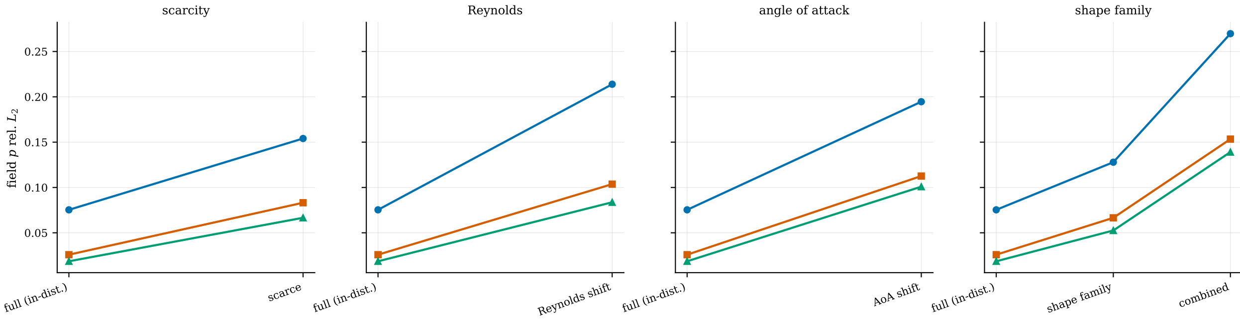
—●— M1 GNN —■— M2 SDF-FNO —▲— M3 Transolver Error vs distribution shift
