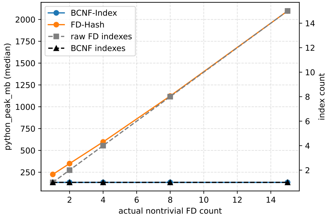
FD count vs memory
