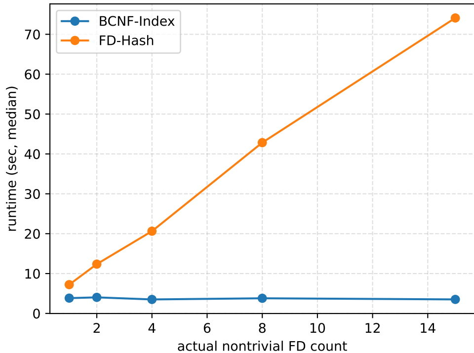
FD count vs runtime
