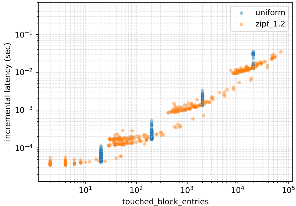
Latency vs touched block entries
