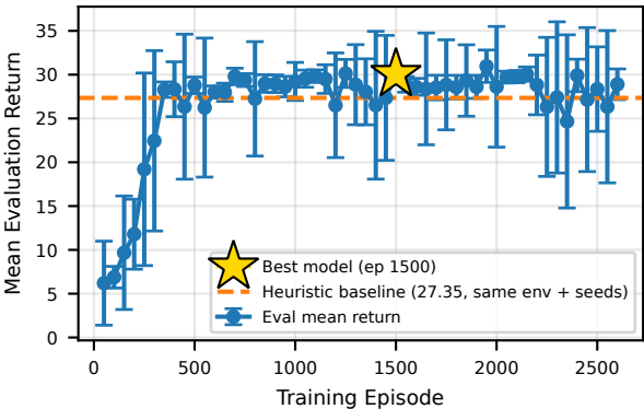
Evaluation Performance During Training
