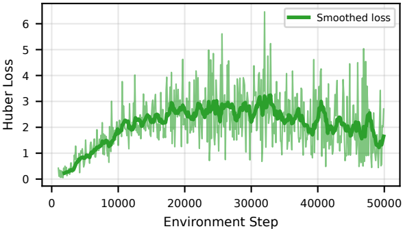
DQN Training Loss
