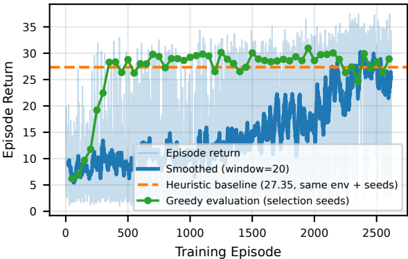
DQN Training Progress vs. Baseline
