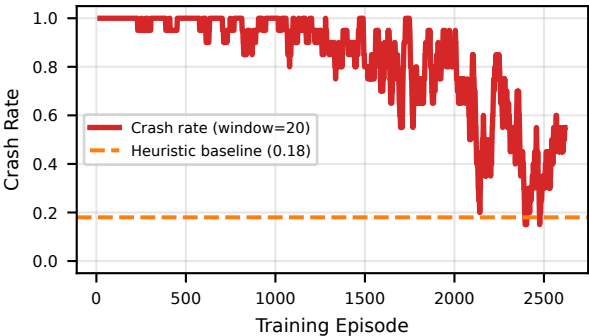
Collision Rate During Training
