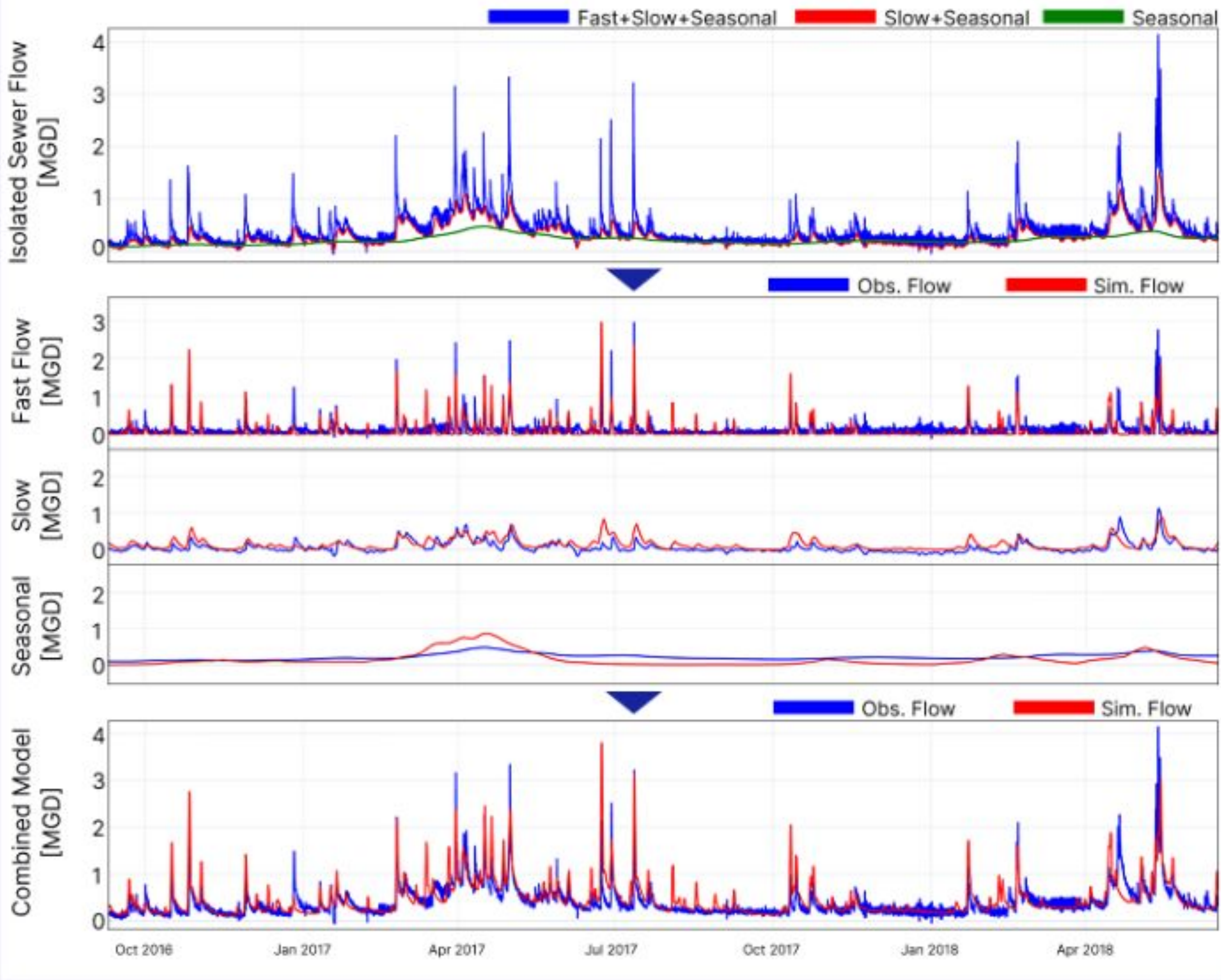
MS0208 Sewer, Observed and Simulated Flow
