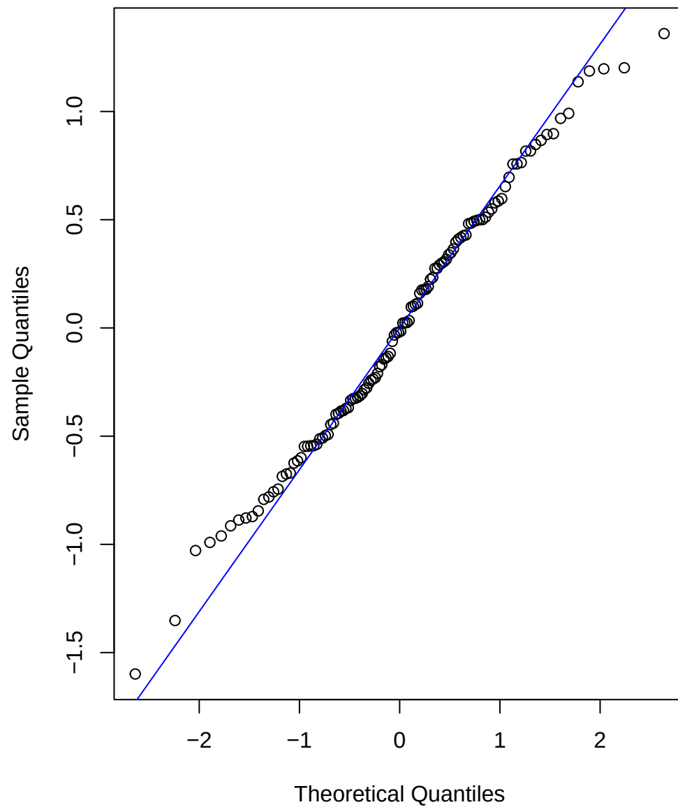
Task 3: residual Q-Q plot
