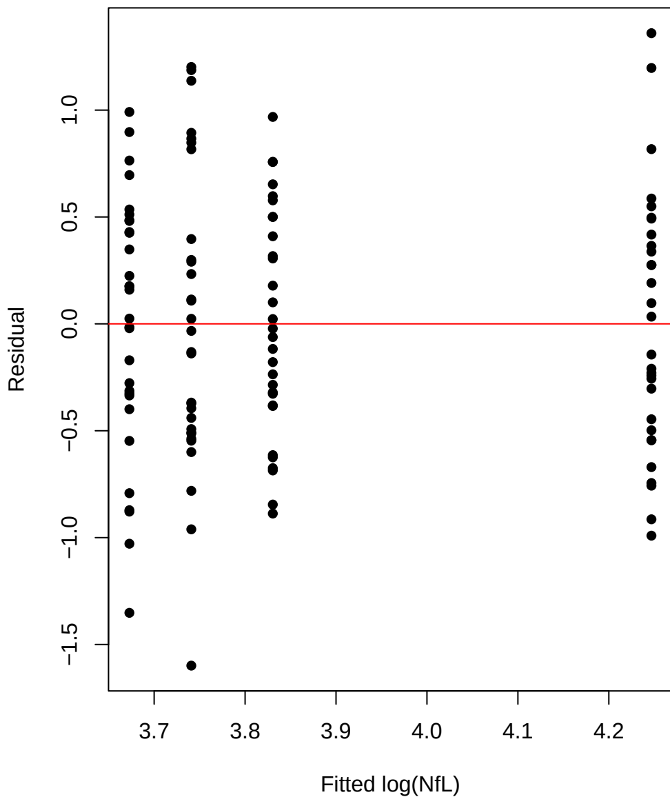
Residuals versus fitted
