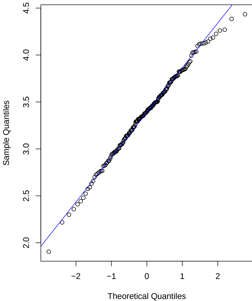
Control: log(NfL)
