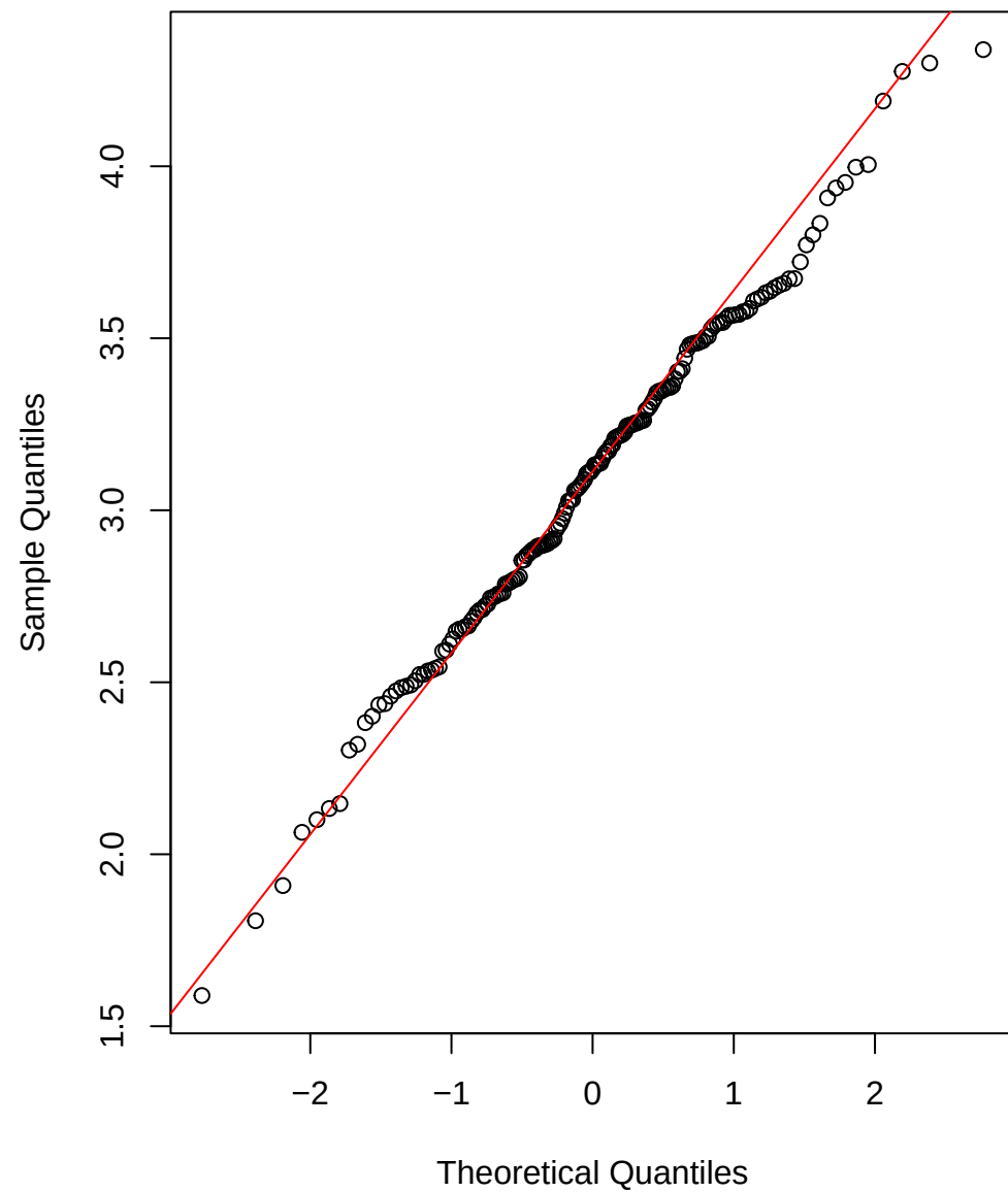
Treatment: log(NfL)
