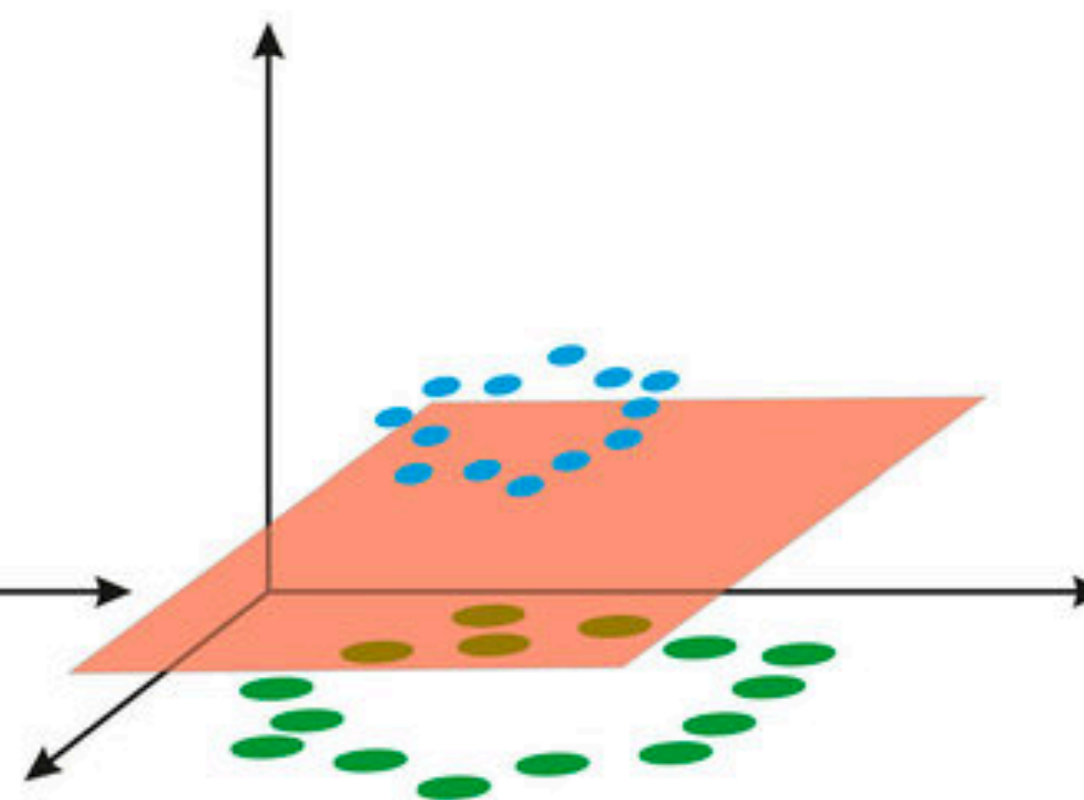
c Separation obtained with a hyperplane in a higher dimensional space (3-D)
