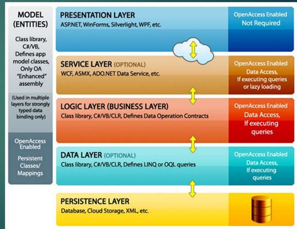
Figura 1. Arhitectura Multi-Tier [3]
