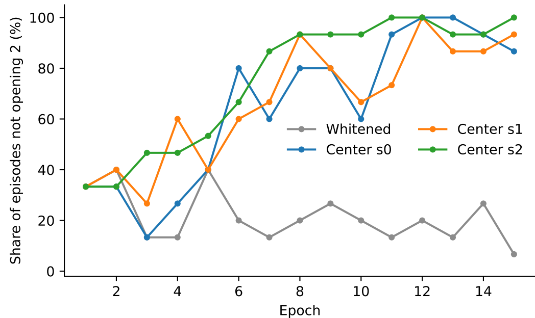
Test A (frozen always-2): leave-opening-2 share
