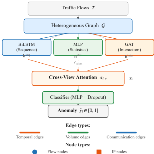
Fig. 1. MGNN architecture.
