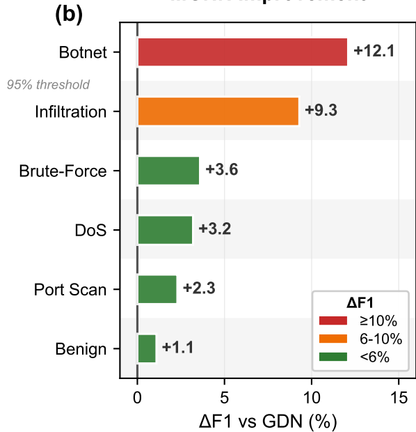
MGNN Improvement
