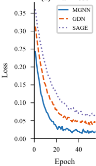
(a) Train loss
