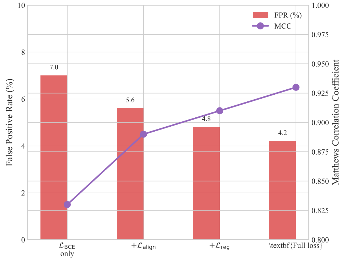
(b) Error Rate and Correlation
