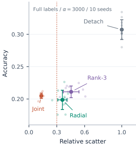
c Survival versus utility
