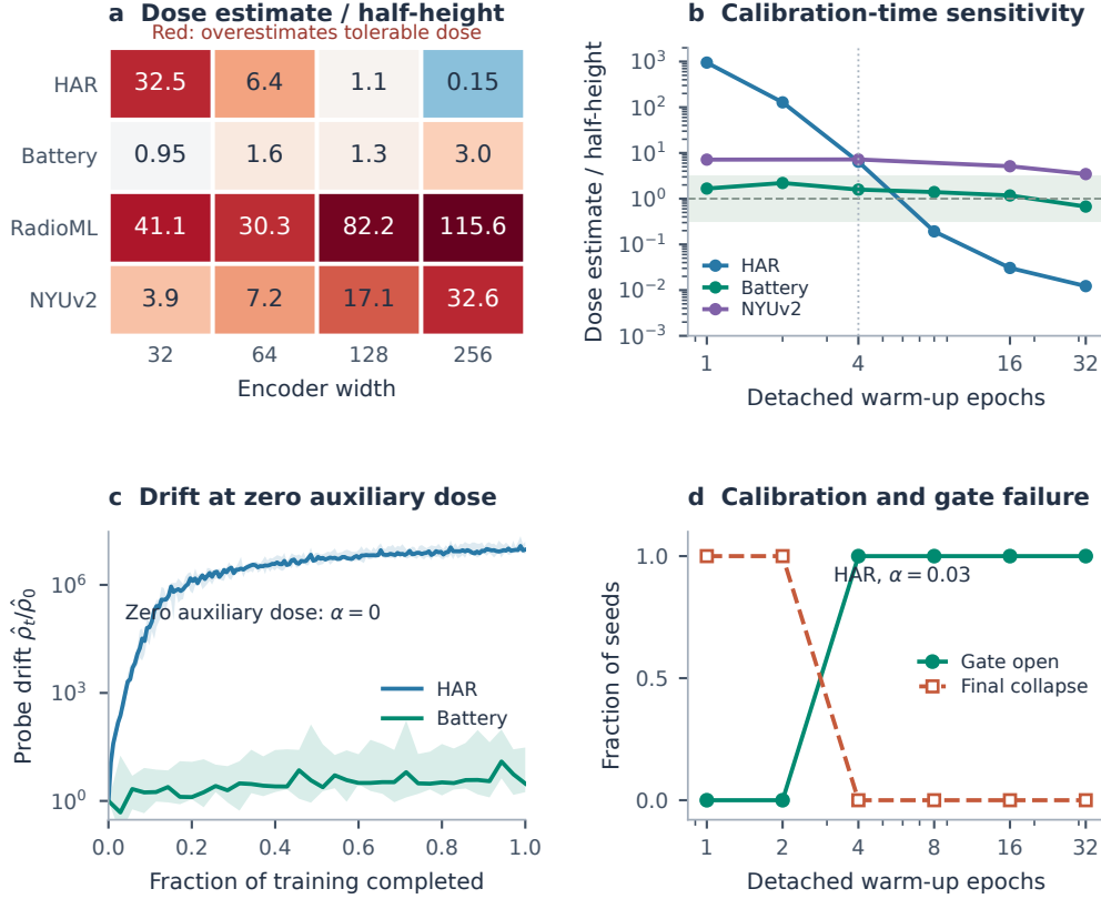
Figure 2: (a) \alpha_{\text{probe}}/\alpha_{1/2} for 16 domain-width cells; all use the controlled toxifier . Red indicates an optimistic dose estimate, blue a conservative one. (b) Changing calibration time changes this ratio at m = 64 ; the shaded factor-3 band is a visual reference, not a confidence interval. Both panels use ten-seed mean probes. (c) At \alpha = 0 , HAR’s probe drifts by orders of magnitude while battery’s remains comparatively stable; median and full range over five seeds, each normalized to its initial value. (d) HAR at \alpha = 0.03 : early calibration leaves all gates closed and all ten runs collapse; at W \geq 4 , all gates open and none collapse. Source values and crossing definitions are in Table 10 and Appendices H.2–H.3.
