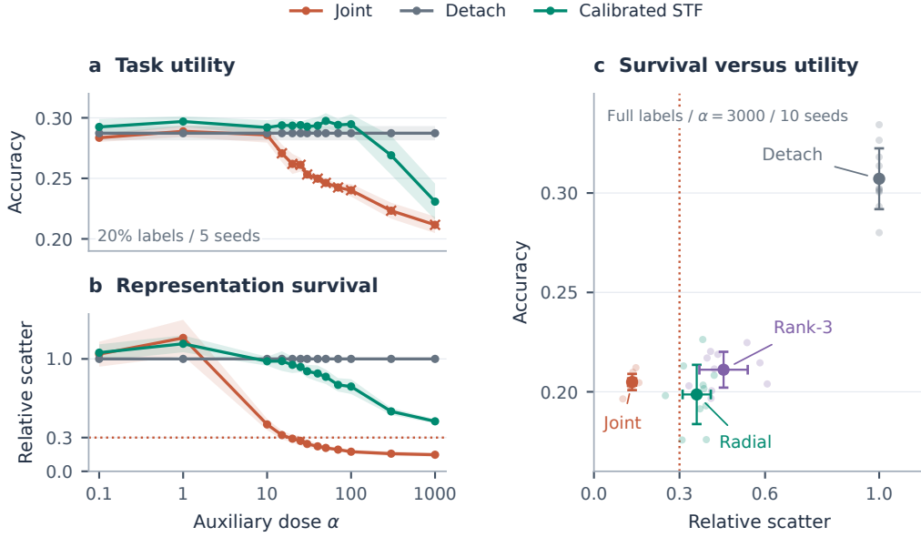
Figure 3: Real RadioML SNR-regression auxiliary. (a,b) At 20% primary labels and width 64, calibrated STF retains a mean accuracy advantage over detachment at intermediate doses; the advantage disappears at extreme doses even while scatter remains above 0.3. Bands are seed standard deviations; crosses mark doses with at least one collapsed joint run. Five unique seeds per dose; duplicate log records are removed. (c) A separate fully labeled, dose-3000 protocol gives a different ordering: rank-3 filtering clears the scatter criterion in all ten seeds, but detachment has higher accuracy. Faint points are seeds; large points and bars show means and standard deviations. The dotted line is the 0.3 scatter criterion.
