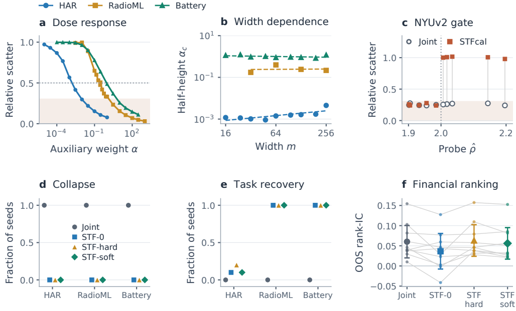
Figure 4: Additional diagnostics across domains. (a) Dose–scatter curves; the half-height crossing differs from the operational 0.3 criterion. (b) Descriptive width trends. (c) Paired NYUv2 boundary outcomes at \alpha = 0.5 . (d,e) Collapse and recovery rates for the archived controlled interventions. (f) Financial rank-IC with temporal folds as the pairing unit. Source protocols and numerical tables are provided in this supplement.
