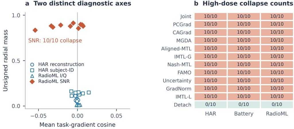
Figure 1: Terminal probes of four real auxiliary heads, ten seeds each. The horizontal coordinate is the mean per-example task-gradient cosine; the vertical coordinate is unsigned radial loading. SNR regression has high loading and 10/10 collapsed endpoints. (b) Operational collapse counts at controlled doses 0.1 (HAR), 3000 (battery), and 10000 (RadioML). All ten optimizers retain collapse. The detached reference uses separate ten-seed controls. Full metrics and control settings are in Table 1.
