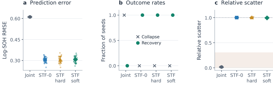
Figure 5: Battery repair under the controlled unified protocol (NASA PCoE, m = 128 , \alpha = 10^4 , 20 seeds per mode). (a) Log-SOH RMSE on a linear axis: the mean decreases from 0.611 to approximately 0.305. (b) Collapse and task-recovery rates. (c) Scatter relative to the same-seed single-task reference; the dotted line marks 1.0 and shading marks the operational collapse region below 0.3. Small points are individual seeds; large markers and whiskers show means and population s.d. These log-SOH errors are not directly comparable with percentage-point SOH errors from the separate battery application.
