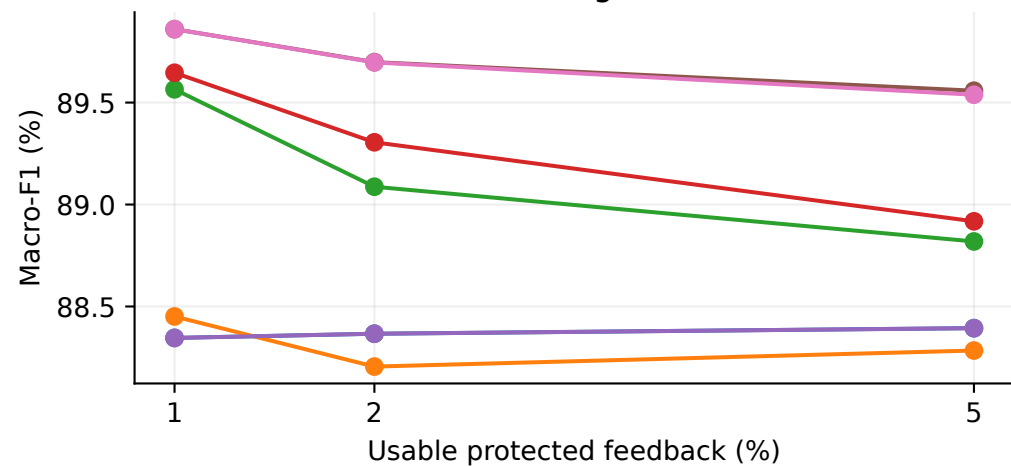
Hellinger
