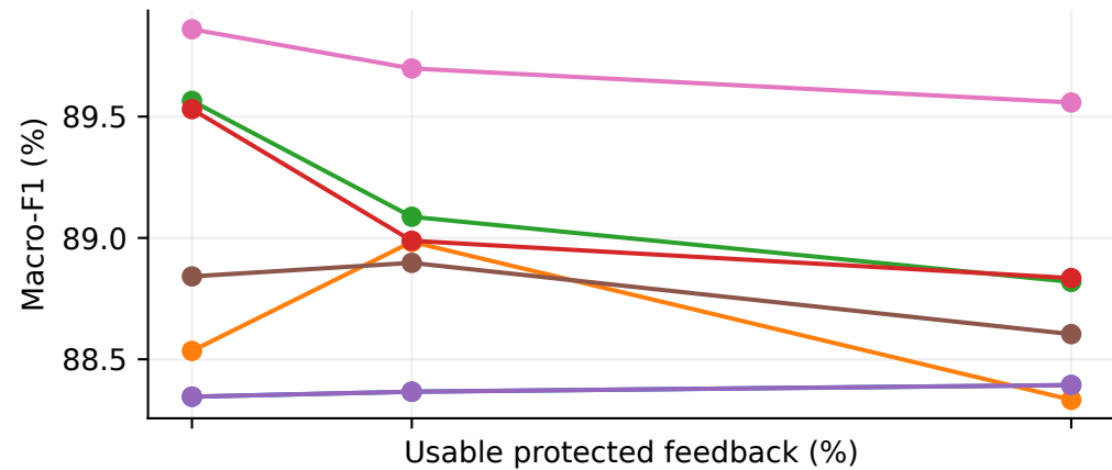
Hellinger
