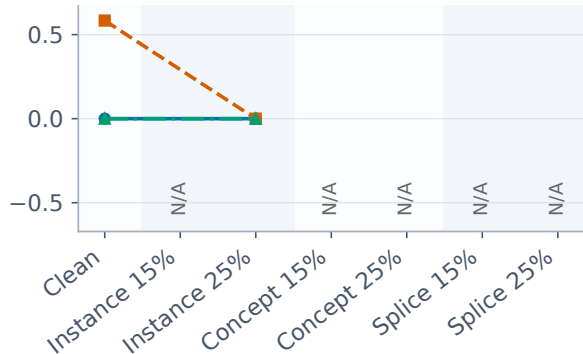
Accuracy (%) difference
