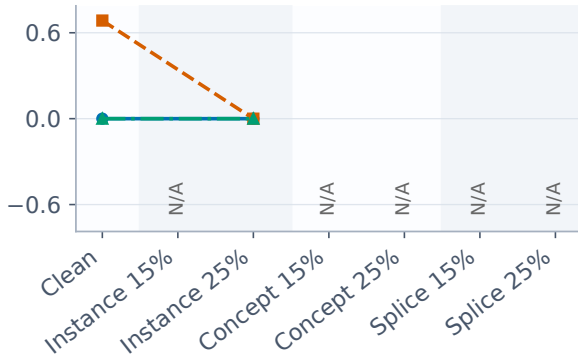
Macro-F1 (%) difference
