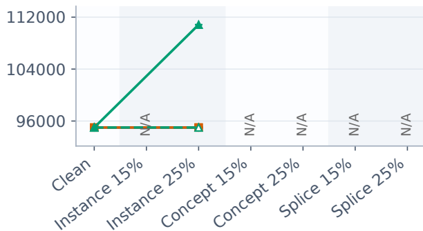
Training work (visits / 100k rows)
