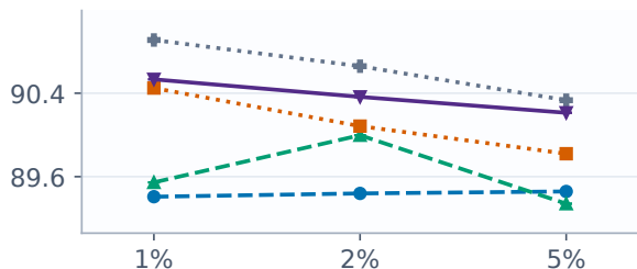
Accuracy (%)
