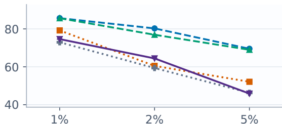
Poison admission (%)
