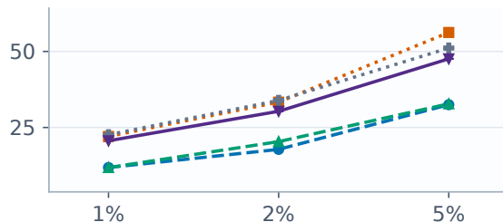
Legitimate withholding (%)
