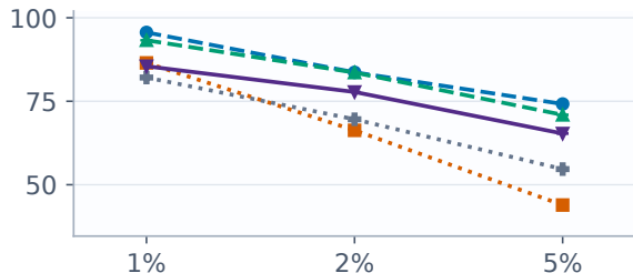
Poison admission (%)
