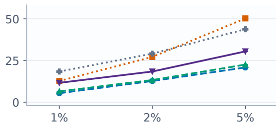
Legitimate withholding (%)
