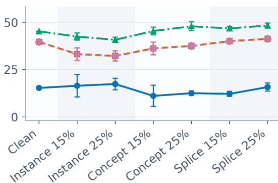
Legitimate withholding (%)
