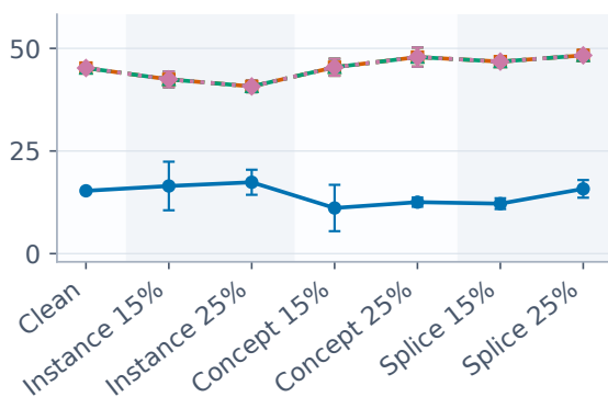
Legitimate withholding (%)
