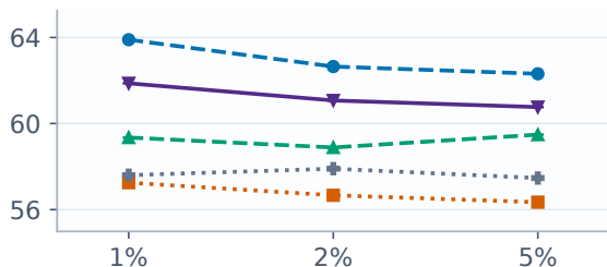
Accuracy (%)
