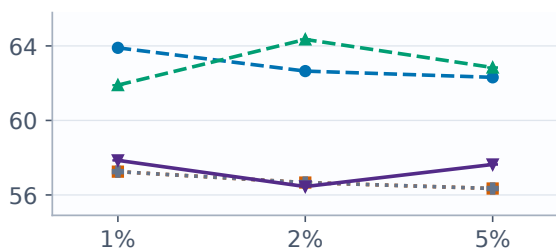
Accuracy (%)
