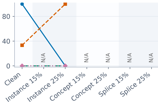
Drift-event recall (%)
