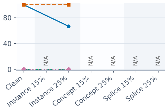
Drift-event recall (%)
