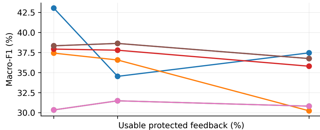
Hellinger
