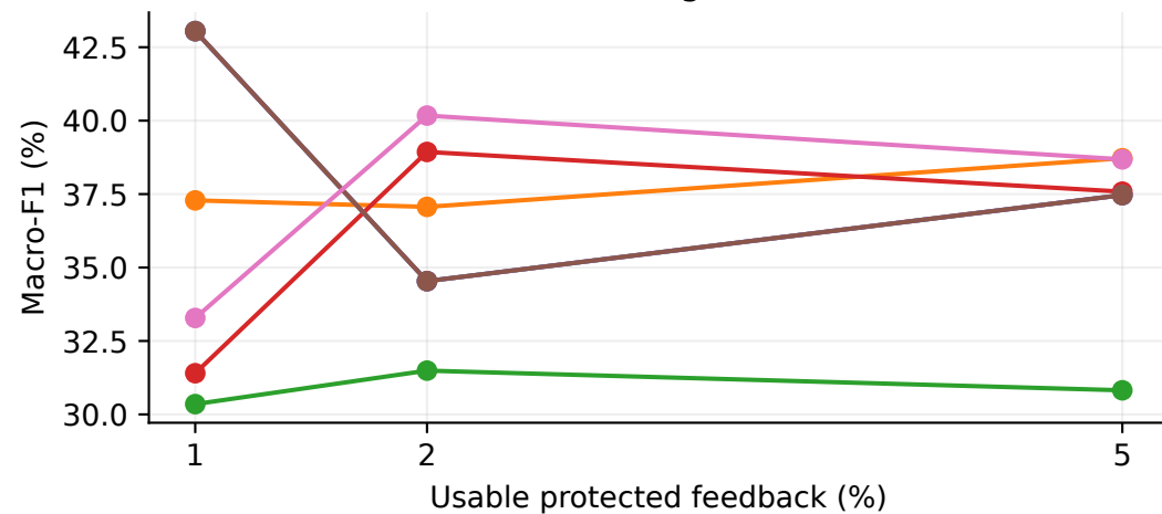
Hellinger
